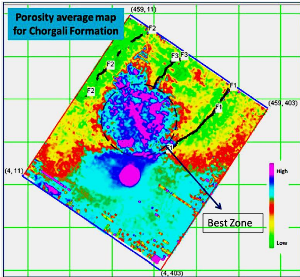
Fig. 9. Average porosity map of Chorgali Formation, plus 10msec average window above.
