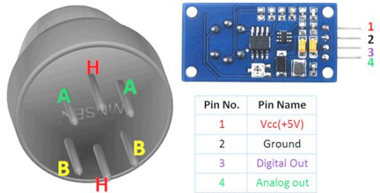
(b) Gas Sensor Pin configuration [4]
